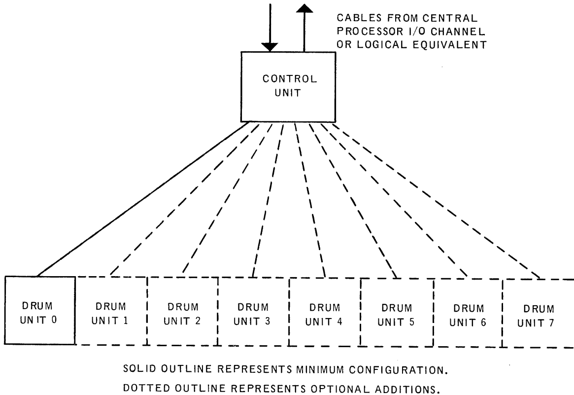
Figure 2-1. Block Diagram of FH-880 Drum Subsystem
