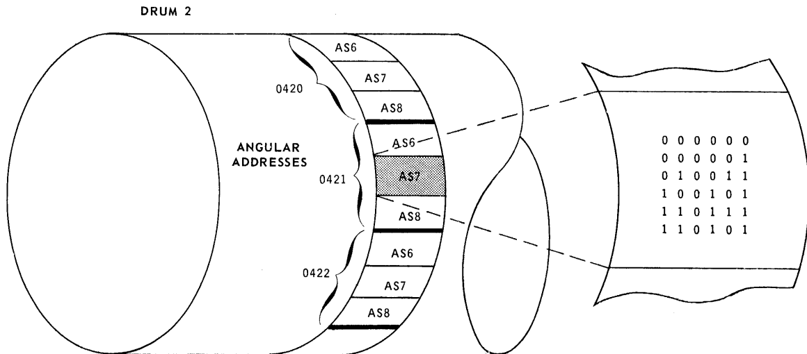
Figure 2-2. Recording Format of FH-880 Drum
